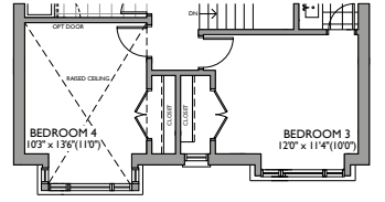
PART. SECOND FLOOR ELEVATION B
