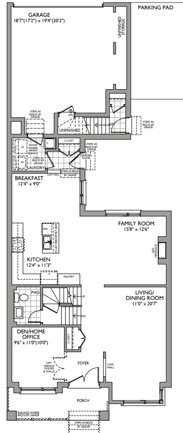
FIRST FLOOR ELEVATION A
