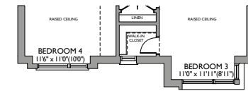
PART. SECOND FLOOR ELEVATION B
