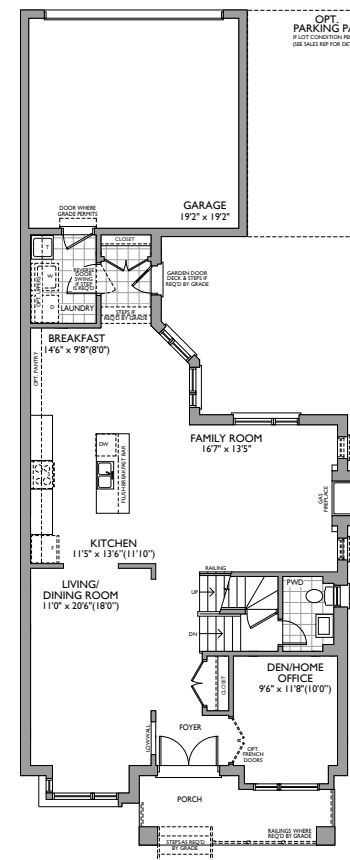
ALTERNATE FIRST FLOOR ELEVATION A
