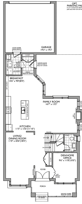
ALTERNATE FIRST FLOOR ELEVATION A
