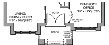
PART. FIRST FLOOR ELEVATION B
