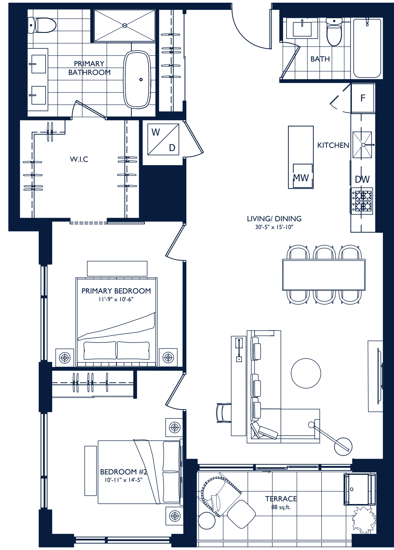
MAIN LEVEL
