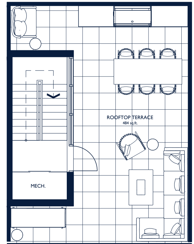
ROOF TOP
