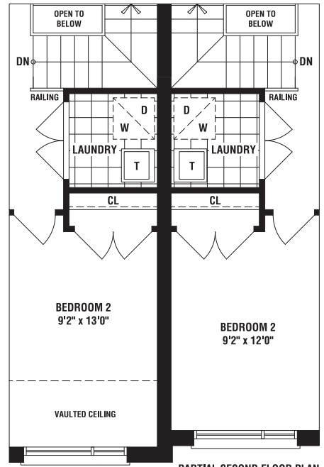
PARTIAL SECOND FLOOR PLAN FOR OPTIONAL LAUNDRY FOR ELEVATION 'B'
