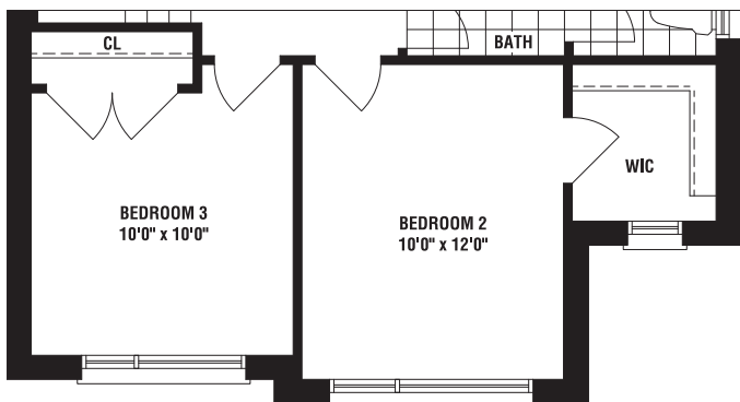
PARTIAL SECOND FLOOR PLAN ELEVATION 'B' 8 FT CEILINGS
