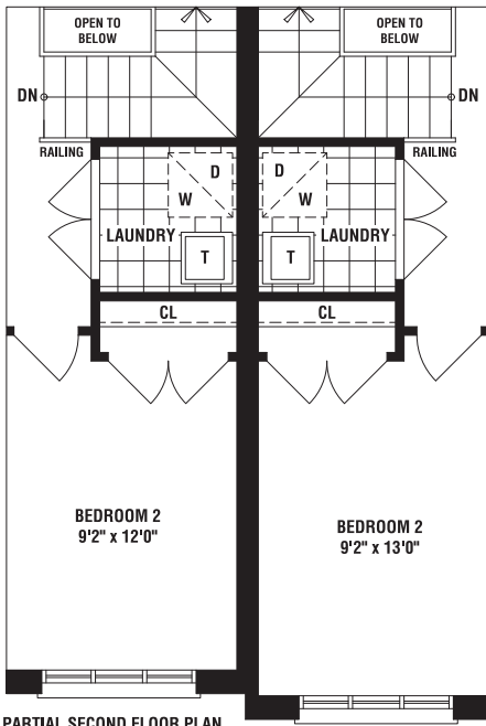
PARTIAL SECOND FLOOR PLAN FOR OPTIONAL LAUNDRY FOR ELEVATION 'A'
