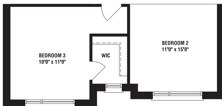
PARTIAL OPT. SECOND FLOOR PLAN ELEVATION 'B' 8 FT CEILINGS
