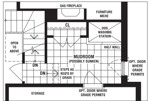
PARTIAL OPT. GROUND FLOOR PLAN W/ DOG WASHING STATION
