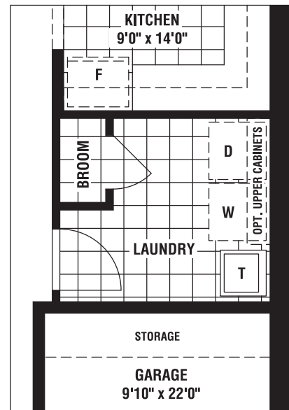
PARTIAL OPT. GROUND FLOOR PLAN FOR OPTIONAL LAUNDRY
