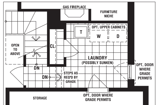
PARTIAL GROUND FLOOR PLAN FOR OPT. LAUNDRY
